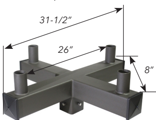
PSS4Q90VTZ 4" 90° quad square vertical tenon
