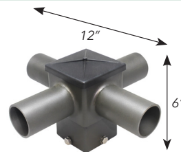
PSS4Q90HTZ Square (quad) horizontal tenon, 90°, bronze. Slips on 4" pole. No adapter needed.
